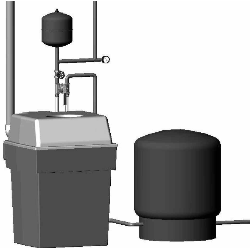
Figure 5 – Plumbing Arrangement
