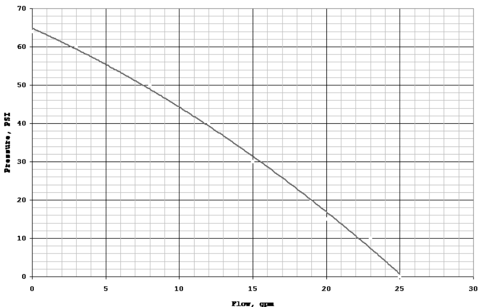
Figure 1. – Pump Curve
