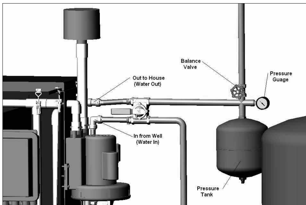
Figure 4 Water Connections
